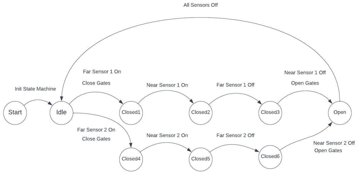
Fig. 13. Gate Control State Machine
