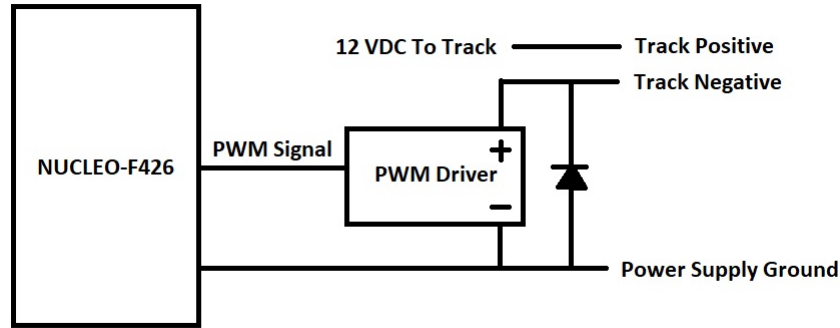
Fig. 3. PWM Circuit
