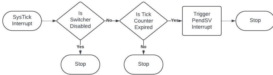
Fig. 7. SysTick Routine
