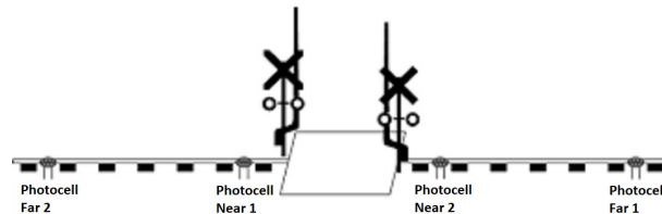
Fig. 12. Crossing Gate Image
