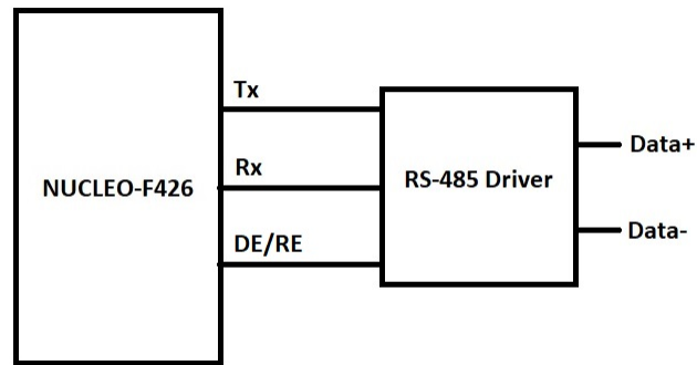
Fig. 4. RS-485 Driver
