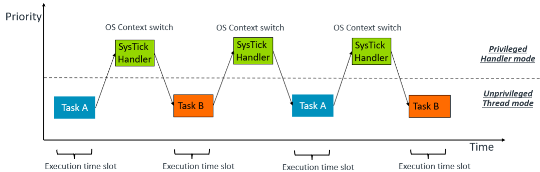
Fig. 6. Preemptive Context Switcher
