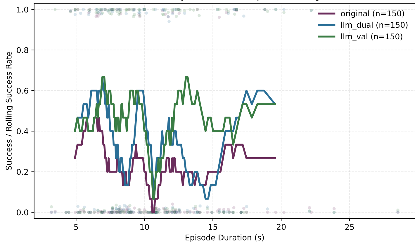
DROID: Time vs Accuracy (all recovered points, rolling window=15)
