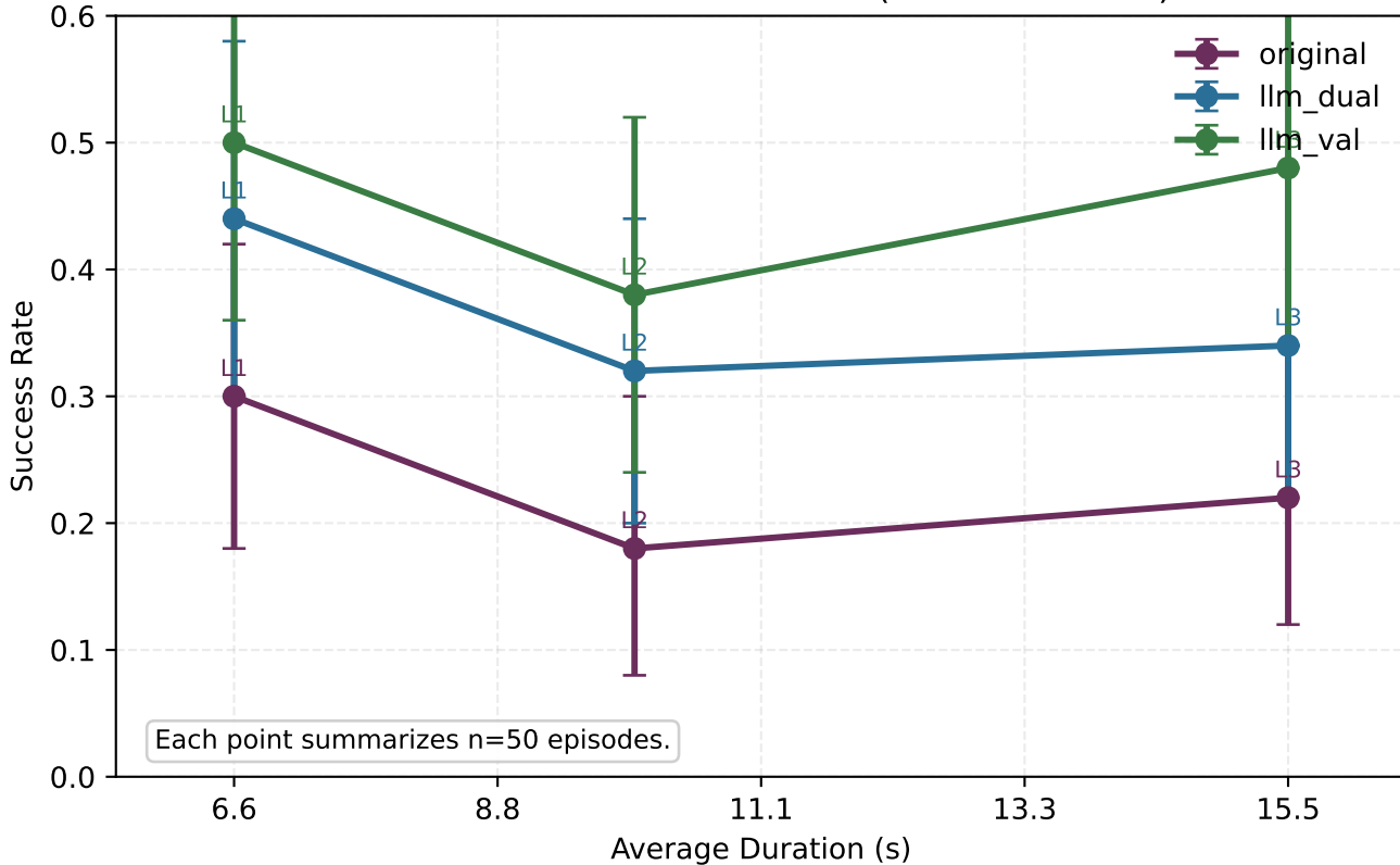
DROID: Time vs Success Rate (All Table Modes)
