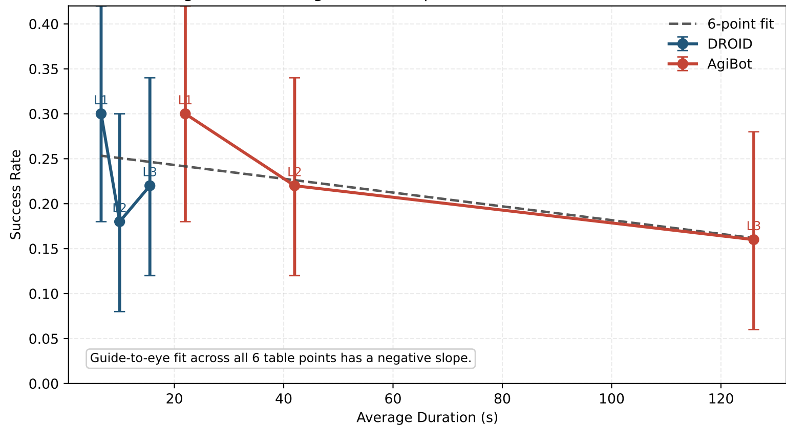
Original Mode: Longer-Horizon Splits Tend to Have Lower Success
