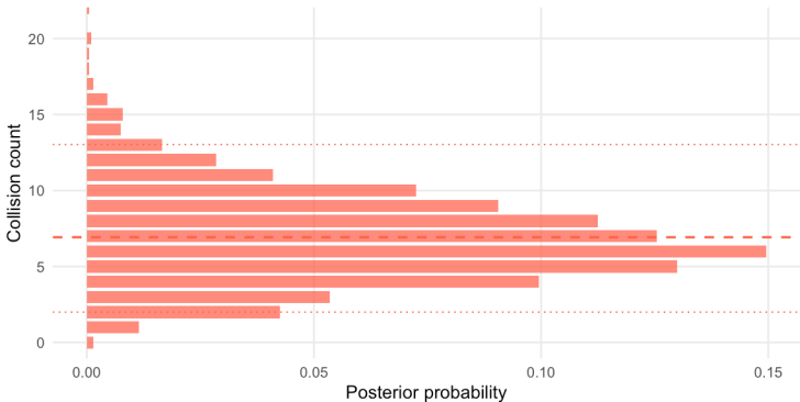
Figure 8: Estimated probabilities of observing different collision counts in the next year
