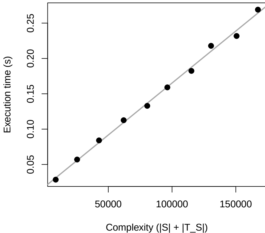
Vectorized scoring complexity R-squared = 0.9962
