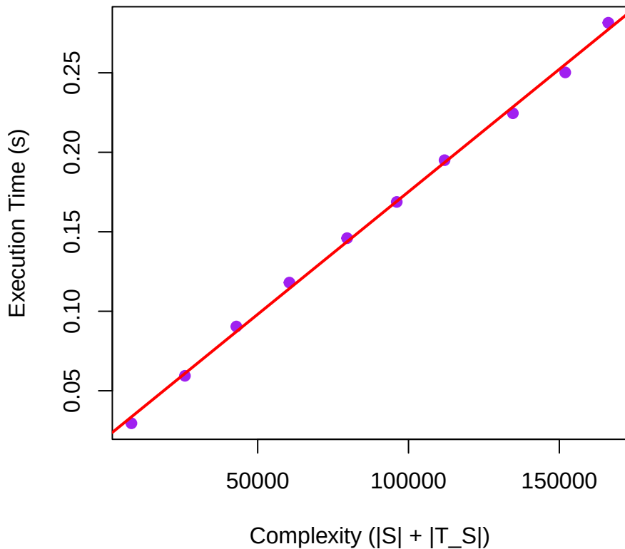
Vectorized Scoring Complexity R-squared = 0.9983
