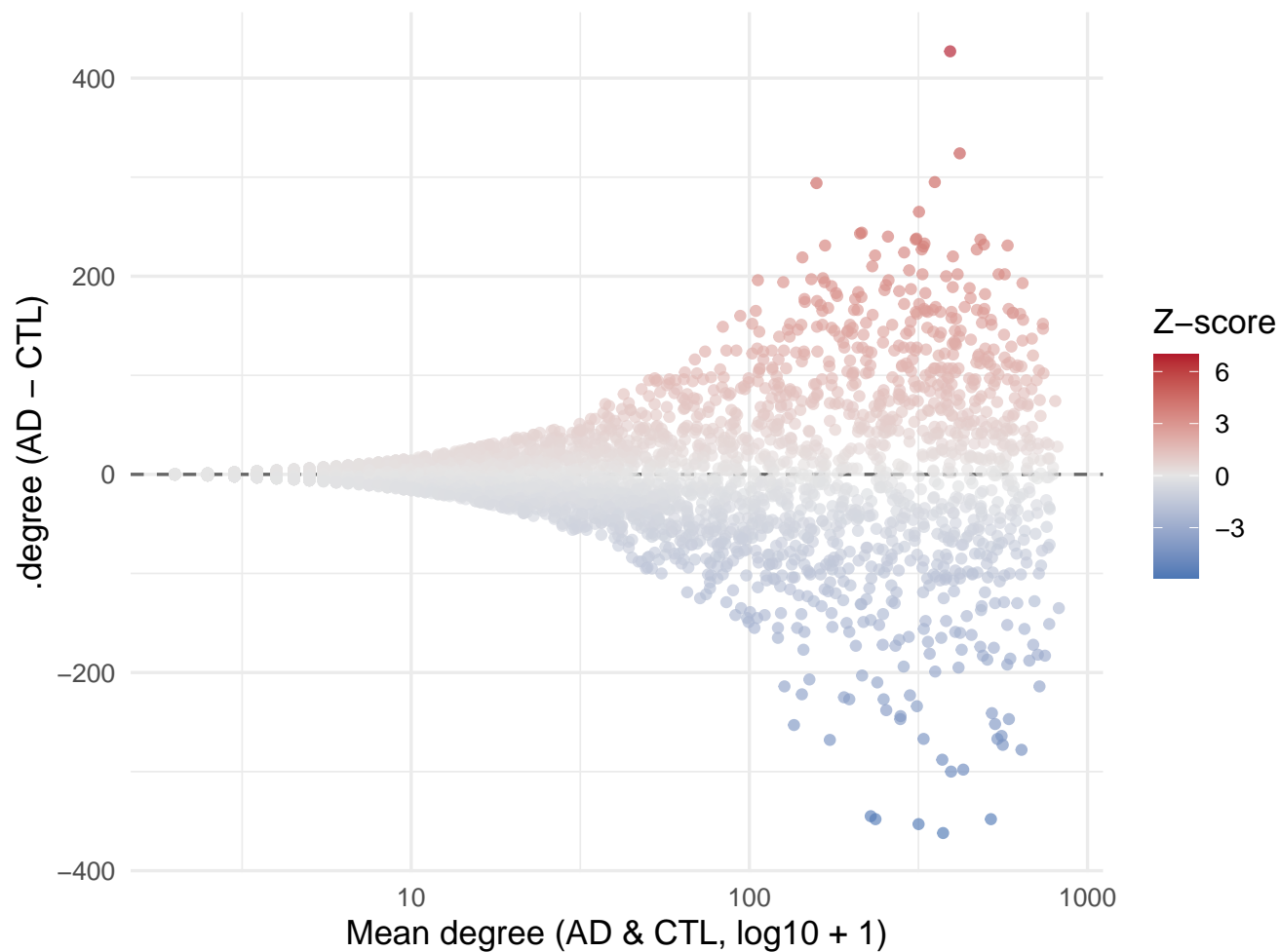
.degree vs mean degree (AD – CTL, common genes)
