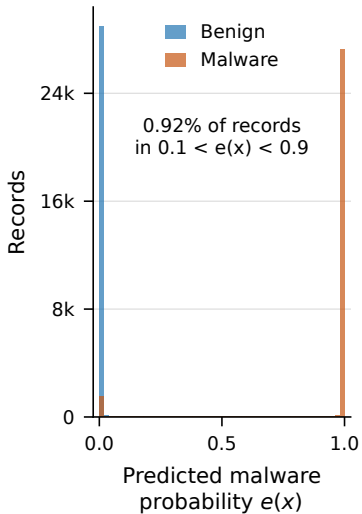
(a) Out-of-fold class probabilities
