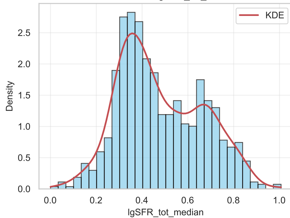
Distribution of lgSFR_tot_median
