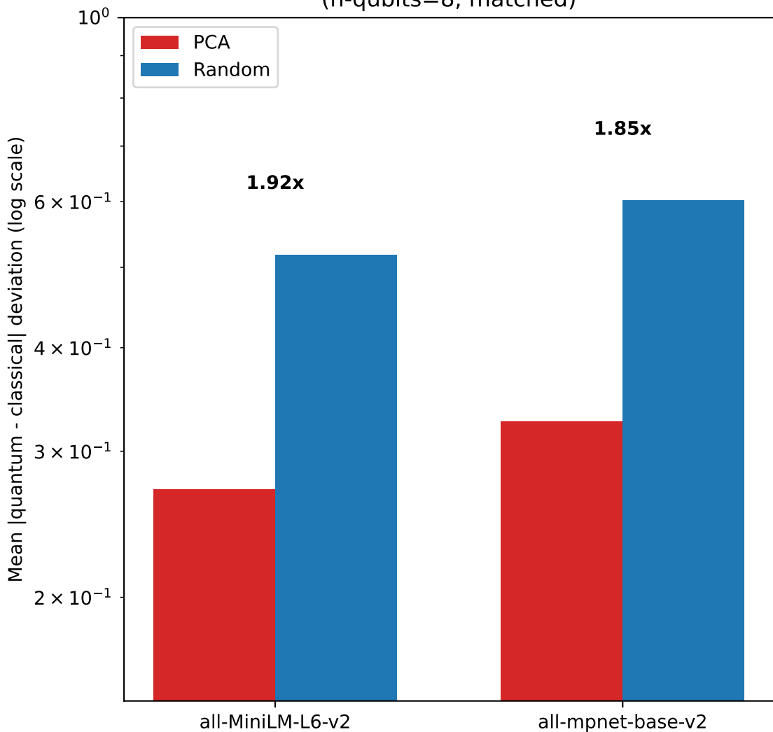
Query-noise dissociation replicates across embedding models (n-qubits=8, matched)
