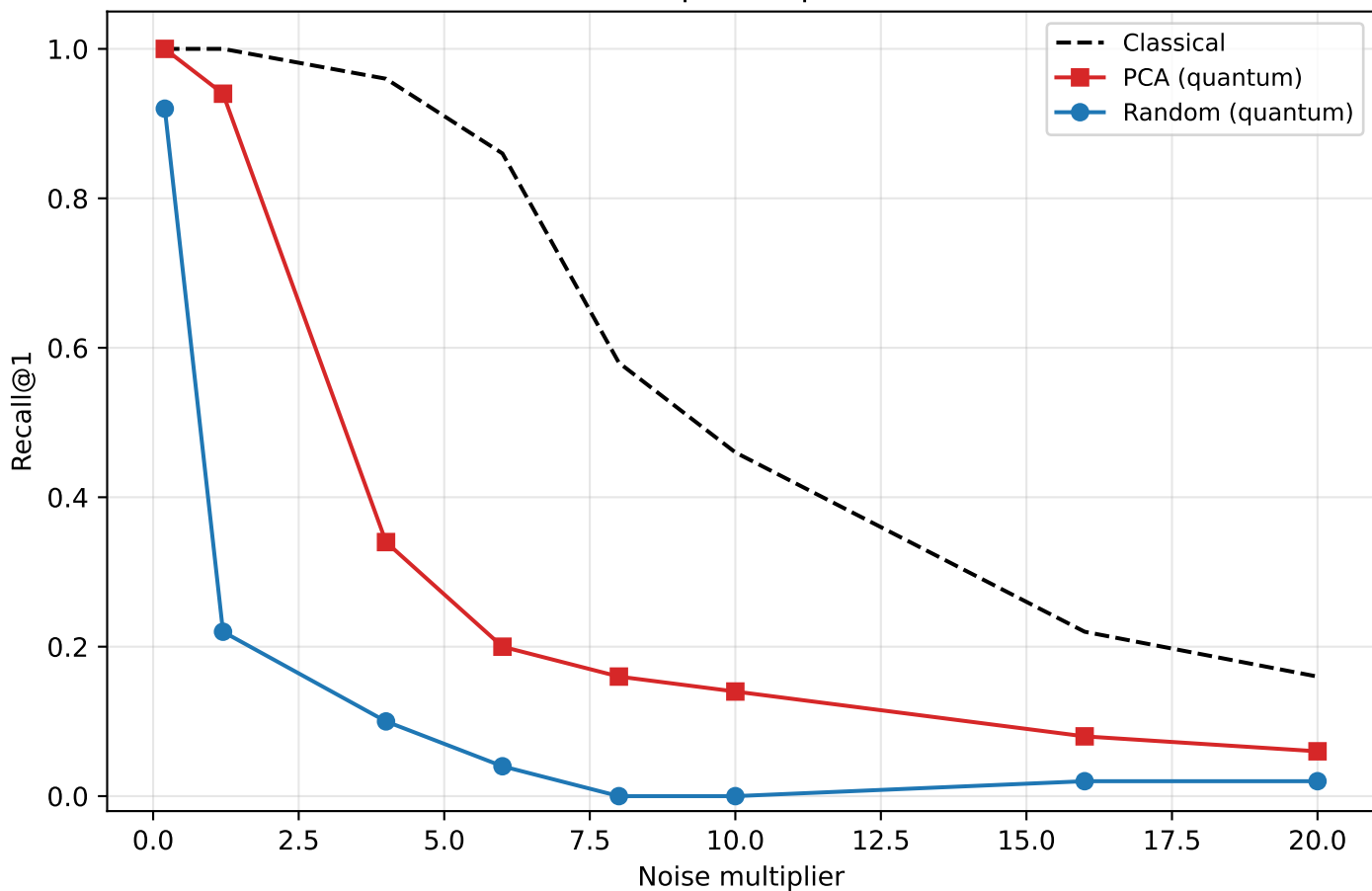
Query-noise sweep: PCA tracks classical at low noise, diverges from multiplier 4.0 onward; random collapses (hard corpus, n-qubits=8)
