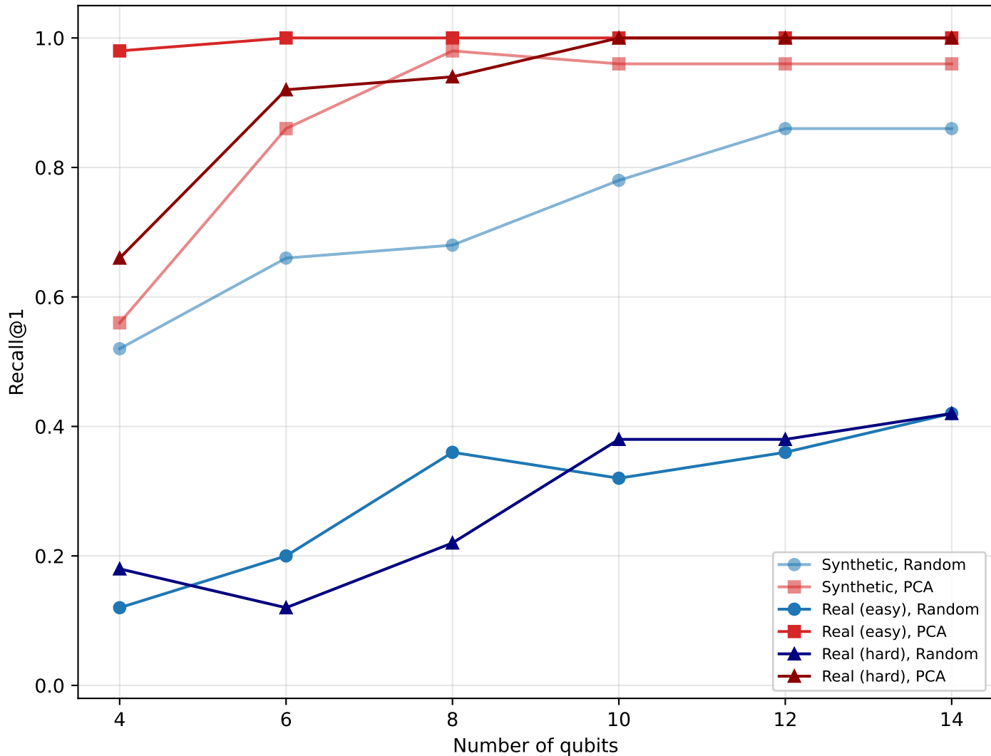
Qubit-count sweep: PCA vs. random projection
