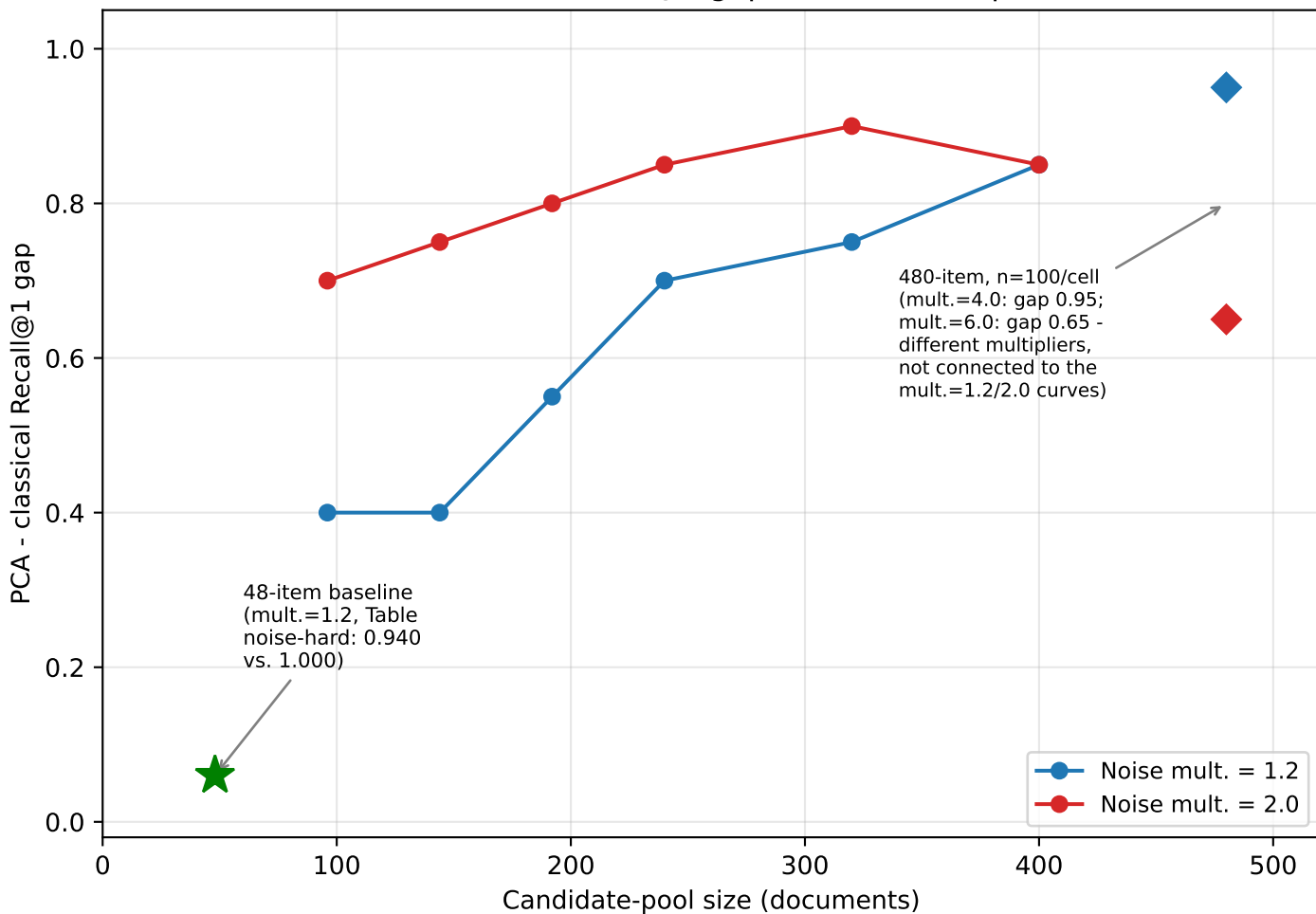
PCA-vs.-classical Recall@1 gap vs. candidate-pool size
