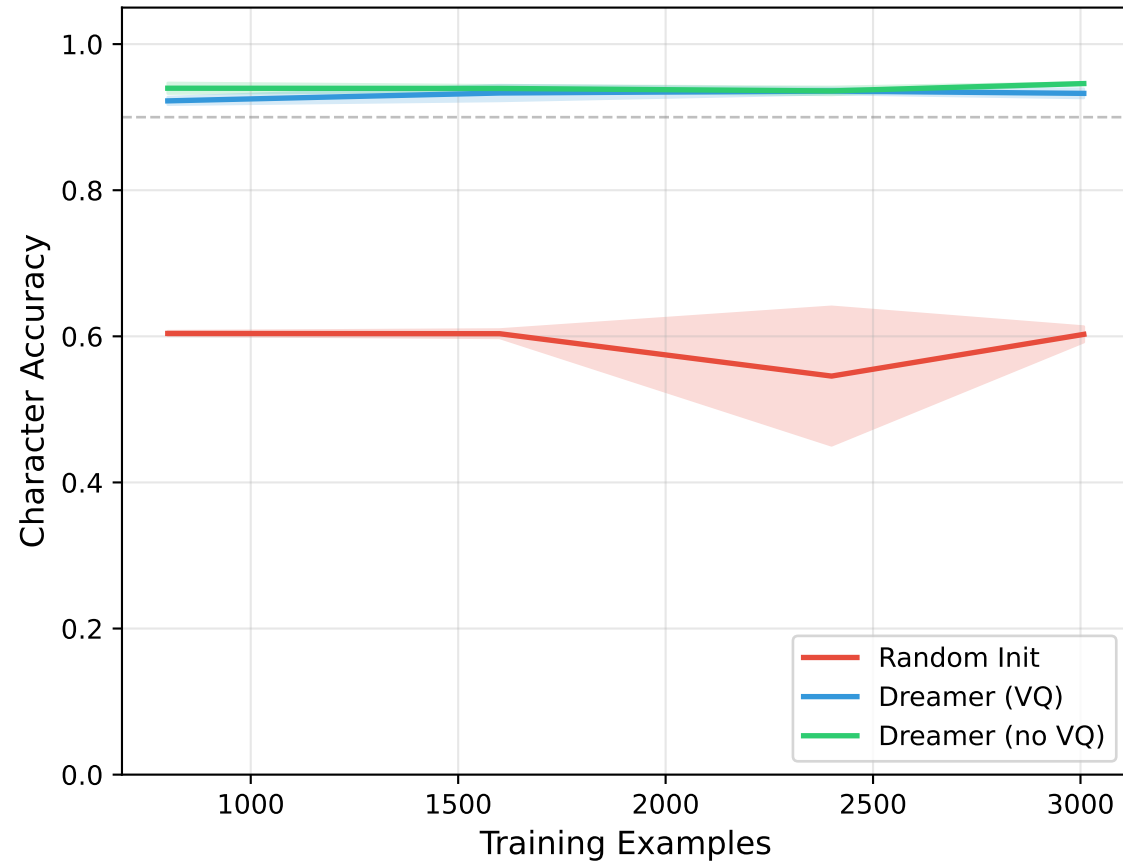
Binary Addition
