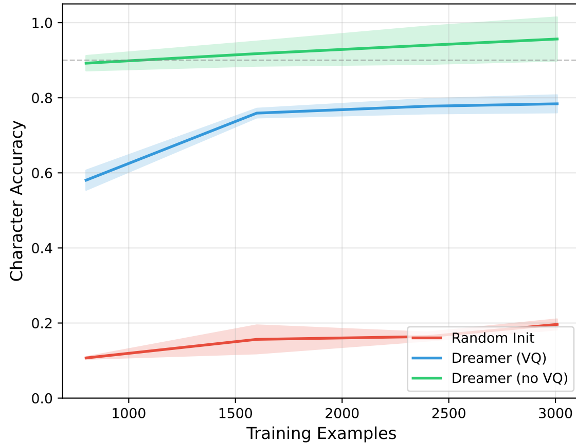
Sequence Reverse
