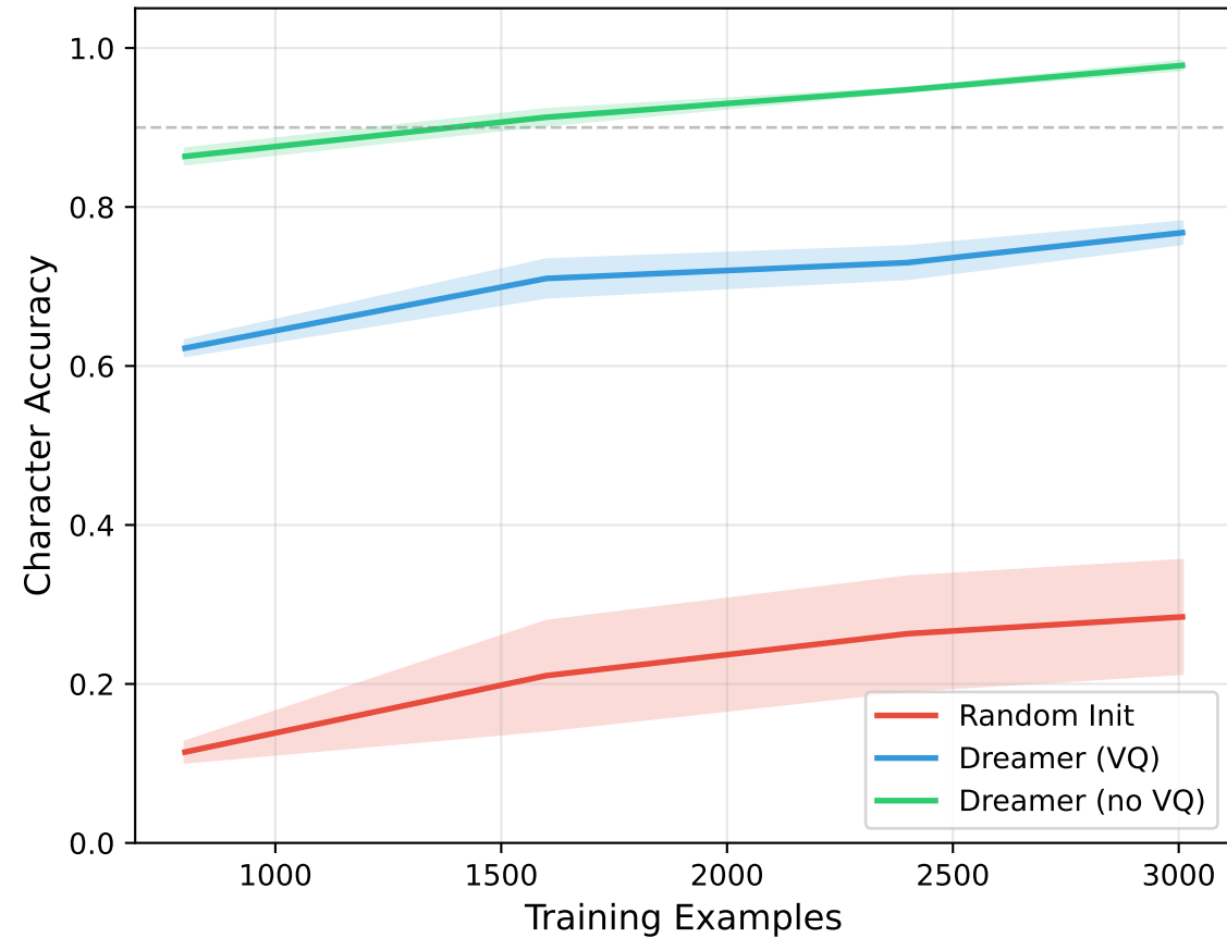
Pattern Completion
