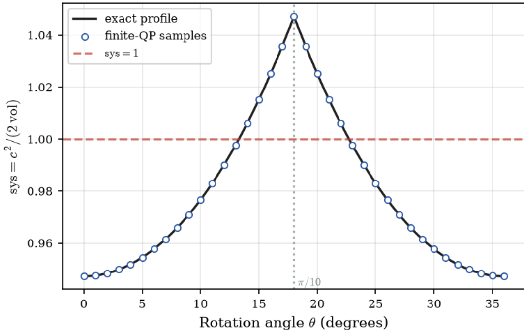
Figure 7: Floating-point finite-QP samples for K_\theta , shown as blue markers, together with the profile proved below. The horizontal line marks the conjectured Viterbo bound. The agreement of the samples with the formula curve is an illustration and discovery check, not an input to the proof.
