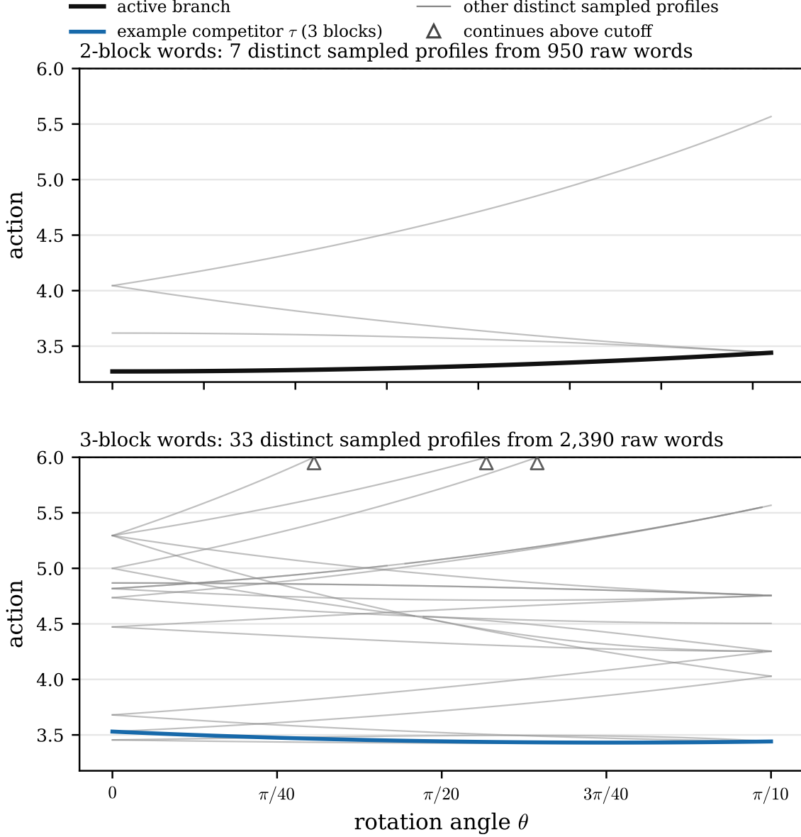
Figure 11: Sampled enumerated KKT-branch landscape. Black marks the active branch and blue the example competitor \tau , whose formula was calculated above. Each gray curve is one of the other distinct sampled profiles defined in the preceding paragraph; the panel headings report the total number of distinct sampled profiles and the number of raw words they summarize. A profile with no admissible sample produces no visible curve. Only consecutive admissible samples are joined. Triangles just below the upper boundary mark curves continuing above the fixed cutoff 6; a gap means that the corresponding word was not numerically admissible at the missing samples. The grid neither certifies feasibility sets nor proves the lower envelope.
