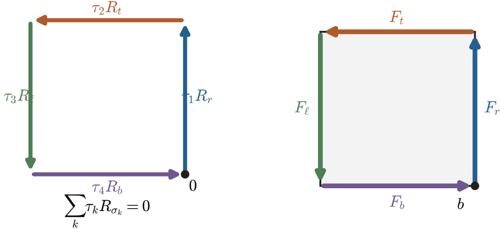
Figure 3: The two layers of finite orbit data in a two-dimensional Hamiltonian analogue. The ordered displacements first form a closed velocity polygon. A translation by a feasible base point then places every segment on its prescribed facet. This is a planar example, not a projection of the four-dimensional orbit; it illustrates only closure and facet realizability.
