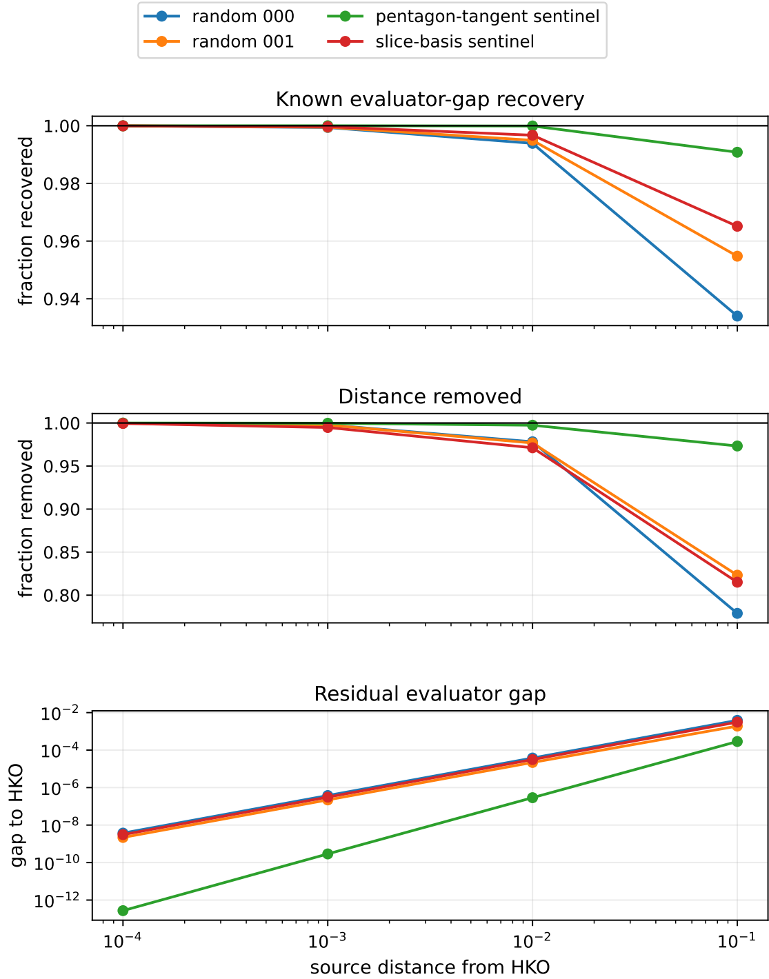
Figure 9: One-step calibration on known perturbations of HKO. From top to bottom, the panels show recovered evaluator gap, removed distance, and residual evaluator gap.
