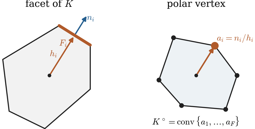
Figure 2: Facet normalization and polarity in a planar model. The supporting line \langle n_i, x \rangle = h_i becomes \langle a_i, x \rangle = 1 after setting a_i = n_i/h_i , and that row is a vertex of the polar polygon. The same facet–polar-vertex correspondence holds in four dimensions; the planar metric proportions are specific to this example and are not part of the duality statement.
