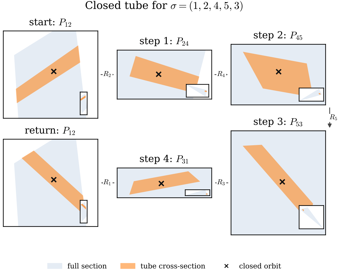
Figure 6: The same word in successive local sections. Each panel plots in a Euclidean-orthonormal basis for the corresponding affine two-plane. The affine origins and orientations are chosen independently for distinct sections; the underlying exact vertices and inequalities remain in the raw construction chart and are not plotted as if they used the orthonormal coordinates. Main panels are tube-focused; each inset locates the colored tube cross-section inside the full blue section. The start and return panels share a frame and plot limits. The arrows show the affine passages, and the black cross returns to its initial coordinates.
