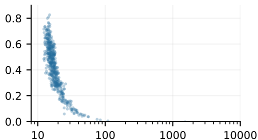
Generic: 12 facets
