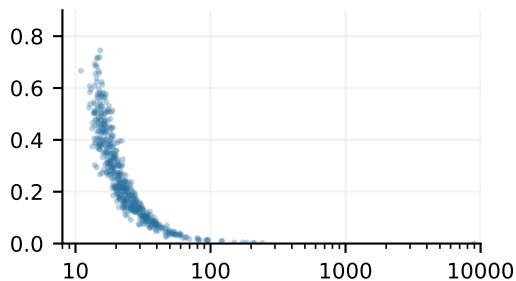
Generic: 10 facets
