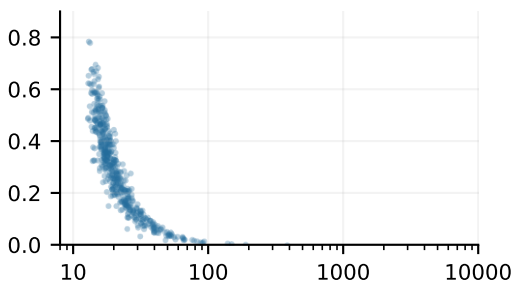
Generic: 11 facets
