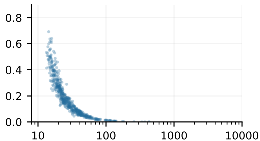
Generic: 8 facets
