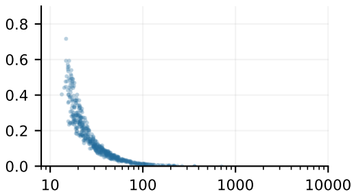
Generic: 7 facets
