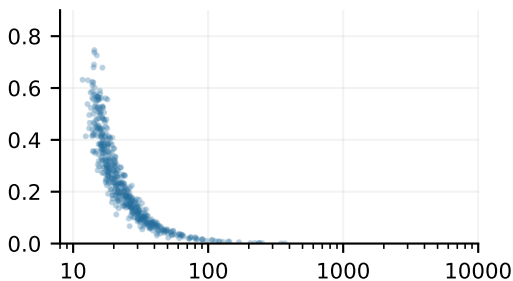
Generic: 9 facets
