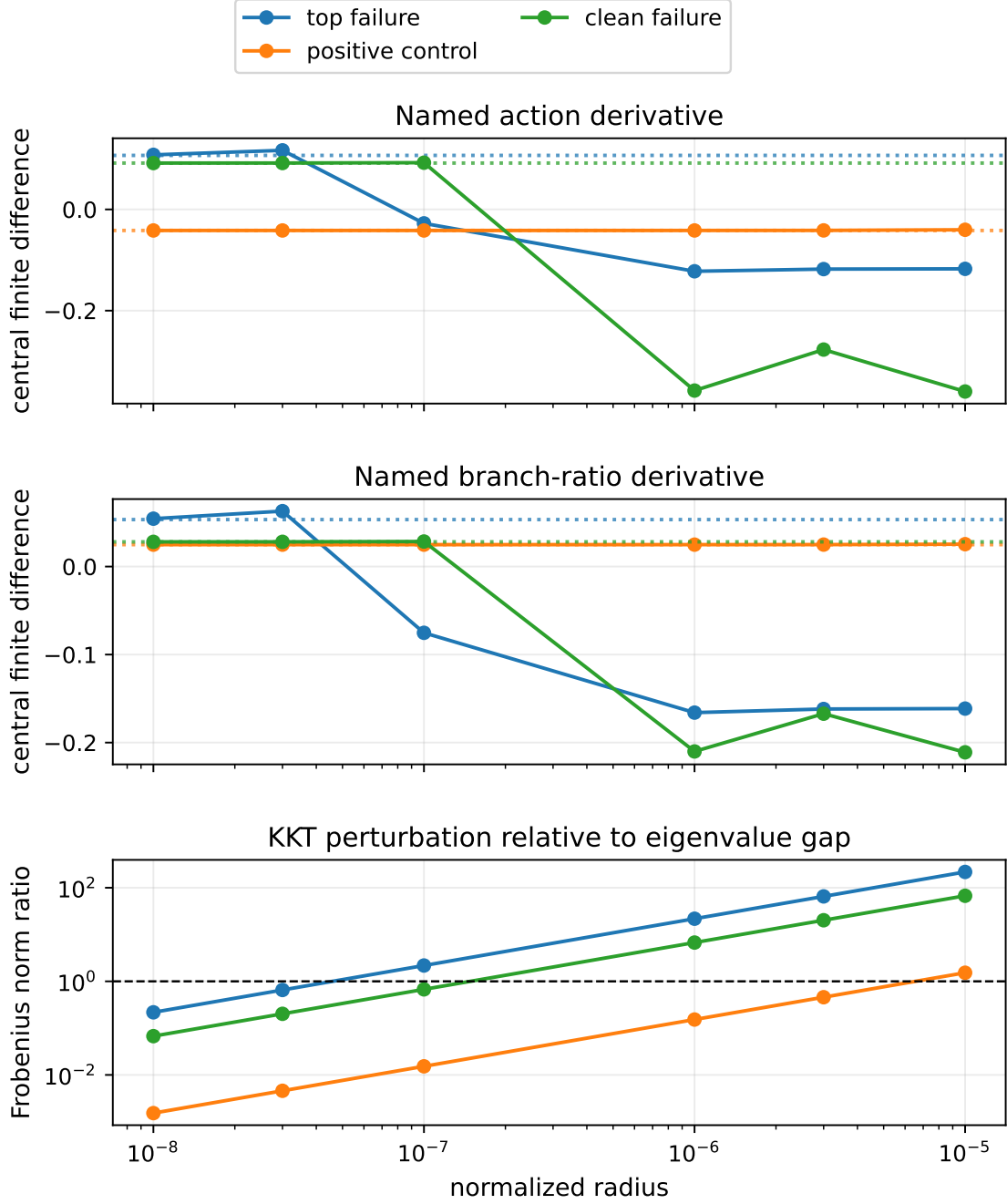
Figure 13: Finite differences for two failed affine proposals and one positive control. Prediction changes regime when the KKT perturbation becomes large relative to the smallest source eigenvalue magnitude (bottom). Dotted lines in the top two panels are the analytic derivatives.
