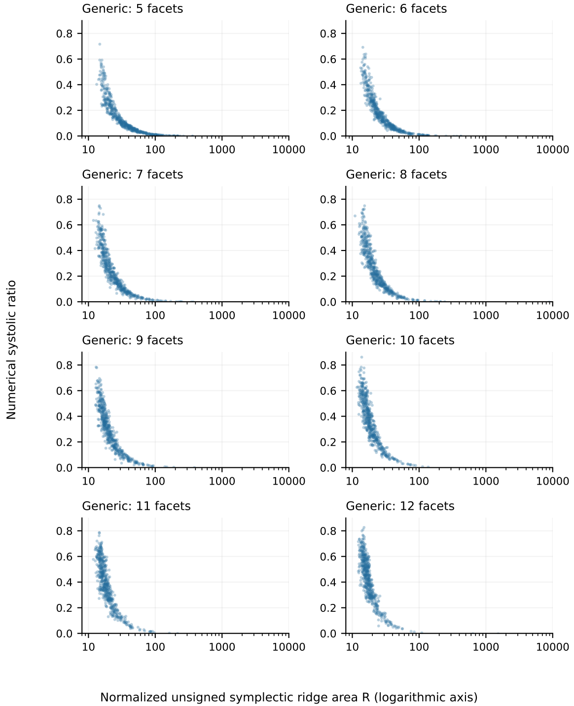
Figure 8: Ridge area and numerical systolic ratio for the 4,096 generic polytopes, separated by facet count. Each point is one body; the horizontal axis is logarithmic. All original numerical values are retained (Appendix A.3).
