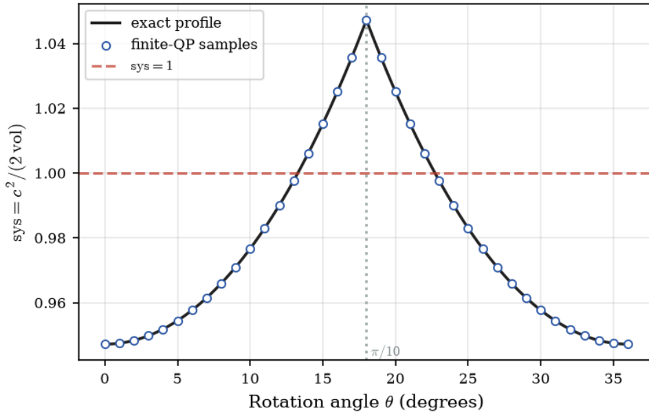
Figure 10: Systolic ratios for the rotating pentagon product. The blue markers are numerical evaluations of the finite quadratic programs; the black curve is the formula proved in this chapter. The horizontal line marks \text{sys} = 1 .
