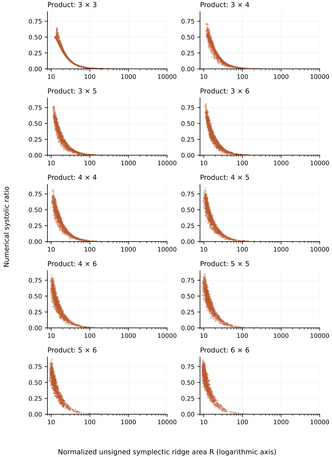
Figure 9: The same comparison for the 10,240 Lagrangian products, separated by factor side counts. Each group contains 1,024 bodies.
