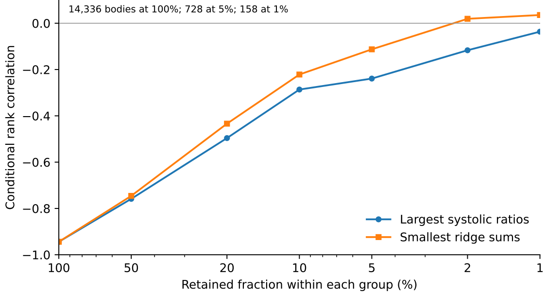
Figure 7: Restricting the original sample by either ridge sum or systolic ratio weakens their inverse association. Within each facet-count or factor-side-count group, retain the indicated fraction, rerank both quantities within that retained group, and compute the pooled Spearman correlation of the group-relative ranks. This is a descriptive conditional analysis of the original data. It does not evaluate a fresh selection rule or identify a geometric cause.
