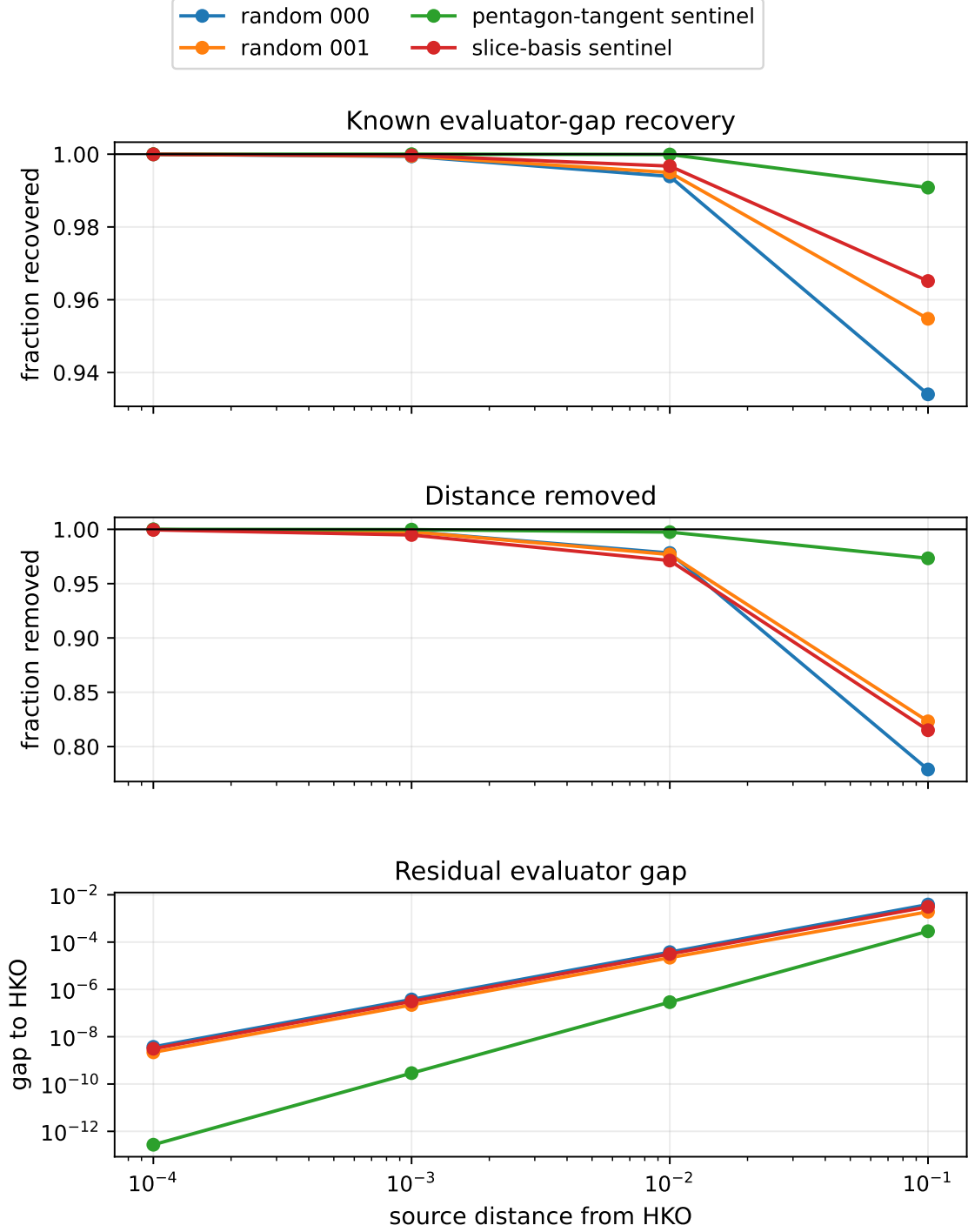
Figure 12: One-step calibration on known perturbations of HKO. From top to bottom, the panels show recovered evaluator gap, removed distance, and residual evaluator gap.
