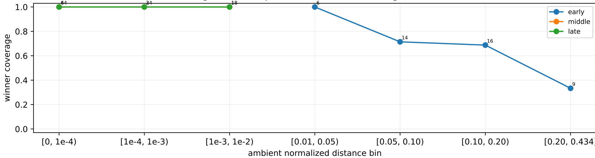
safeguarded-adaptive-d1e-1 (labels are target counts)
