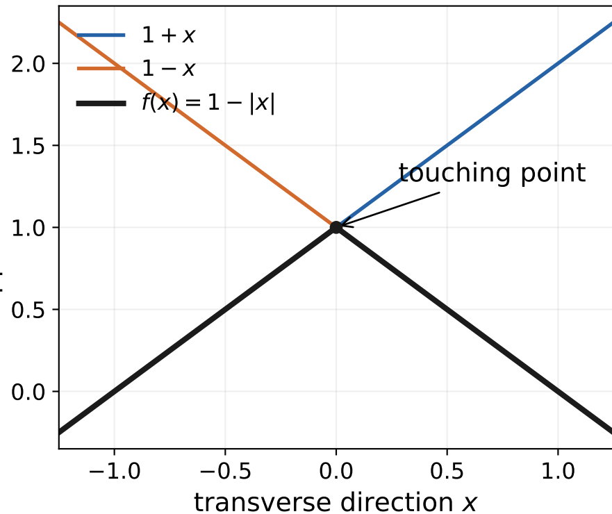
One-dimensional mechanism
