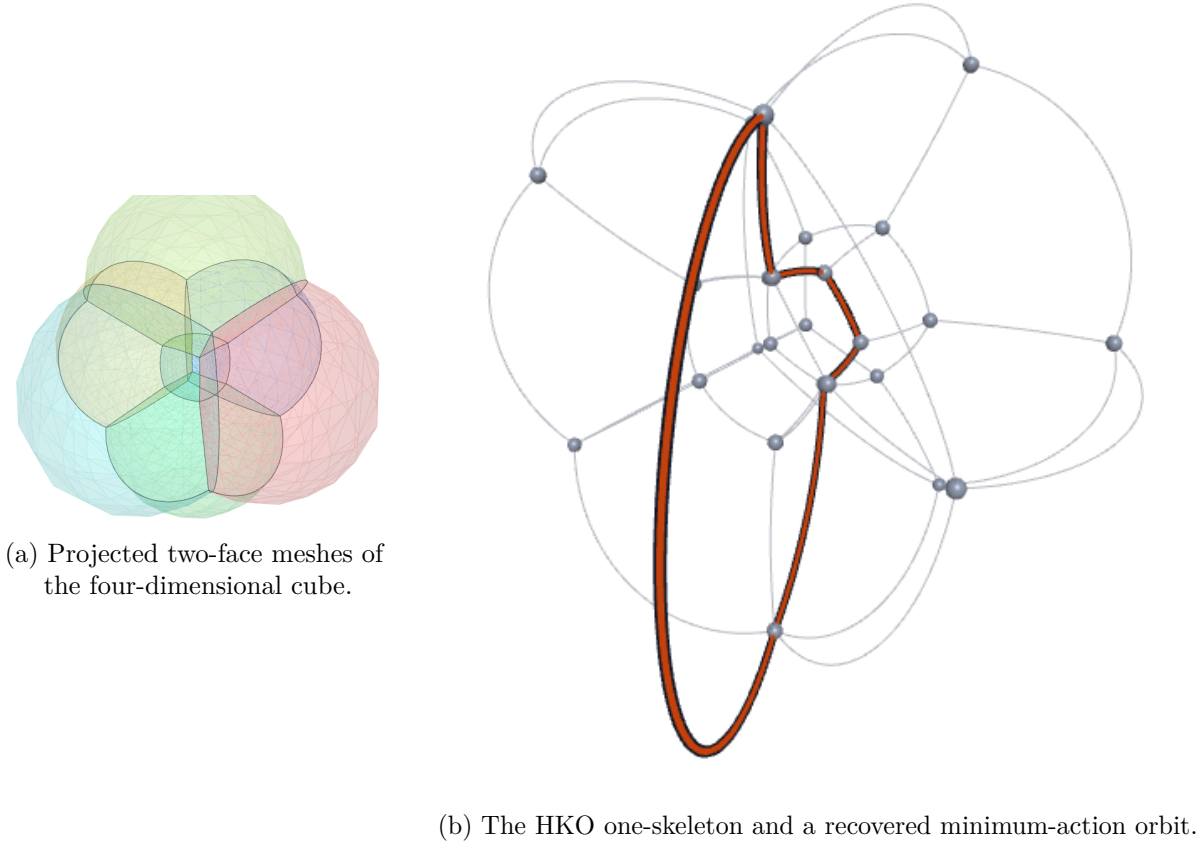
Figure 11: Radial and stereographic views of four-dimensional polytopes. In (a), colour separates projected two-face meshes of the cube. In (b), the grey one-skeleton belongs to the Lagrangian product of two regular pentagons and the dark-outlined orange curve is a recovered six-segment closed Reeb orbit. Both panels use the pole e_4 and omit parts mapped beyond the viewer's clipping radius. They are qualitative explanatory views, not symplectic invariants or proof evidence.
