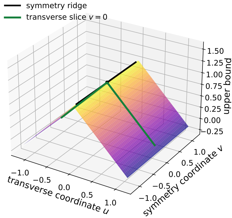
Figure 6: The toy function f(u, v) = 1 - |u| has a strict maximum on the transverse slice v = 0 and is constant along the symmetry coordinate v . Its maxima form the ridge u = 0 . In the HKO proof the symmetry tangent space T has dimension fifteen and the transverse space S has dimension twenty-five. The picture illustrates their roles in the local decomposition.
