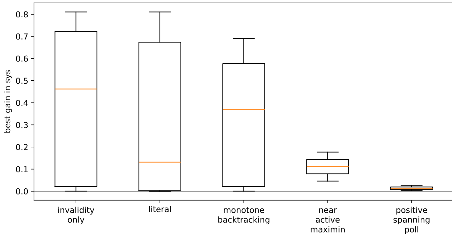
Optimizer suite: retained best gain
