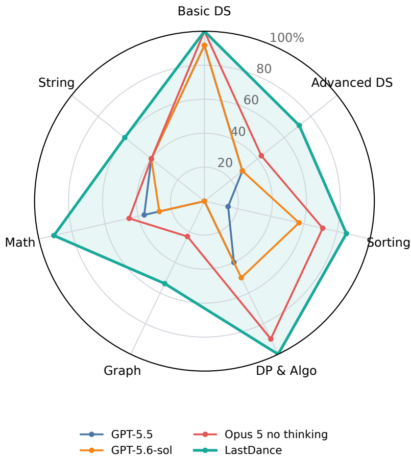
(a) Full-mark rate by AlgoVeri category
