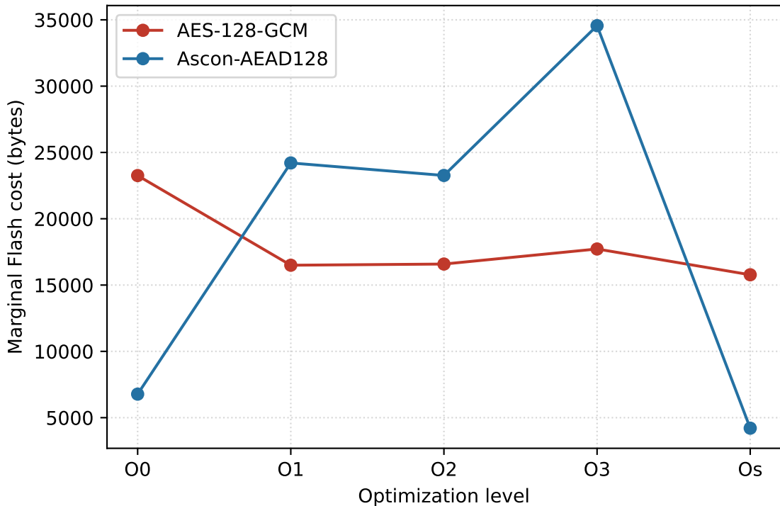
Code size vs optimization level (L476)
