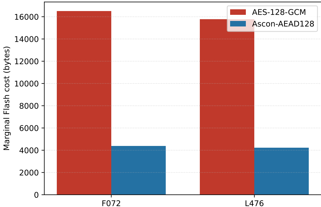
Code-size cost at -Os (over baseline)
