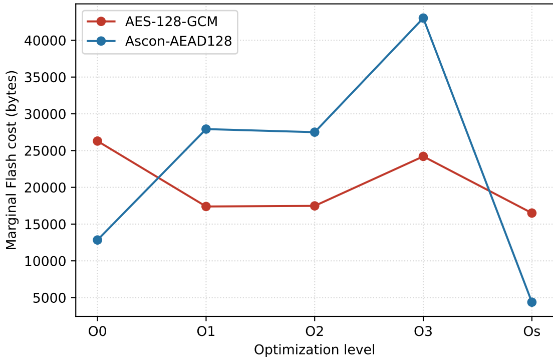
Code size vs optimization level (F072)
