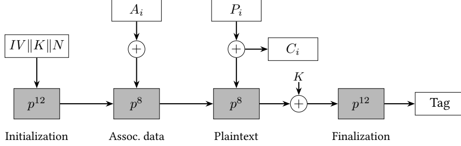
(a) Ascon-AEAD128: a single permutation p absorbs and squeezes a 320-bit state across four phases. Intermediate rounds use p^8 , initialization and finalization use p^{12} .
