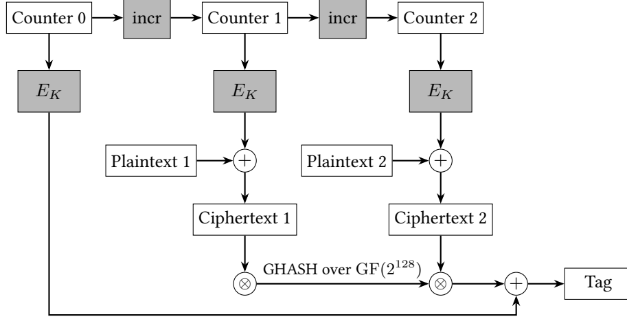
(b) AES-128-GCM: the block cipher E_K runs in counter mode to produce a keystream, and a separate GHASH multiplication in GF(2^{128}) authenticates the ciphertext into the tag.
