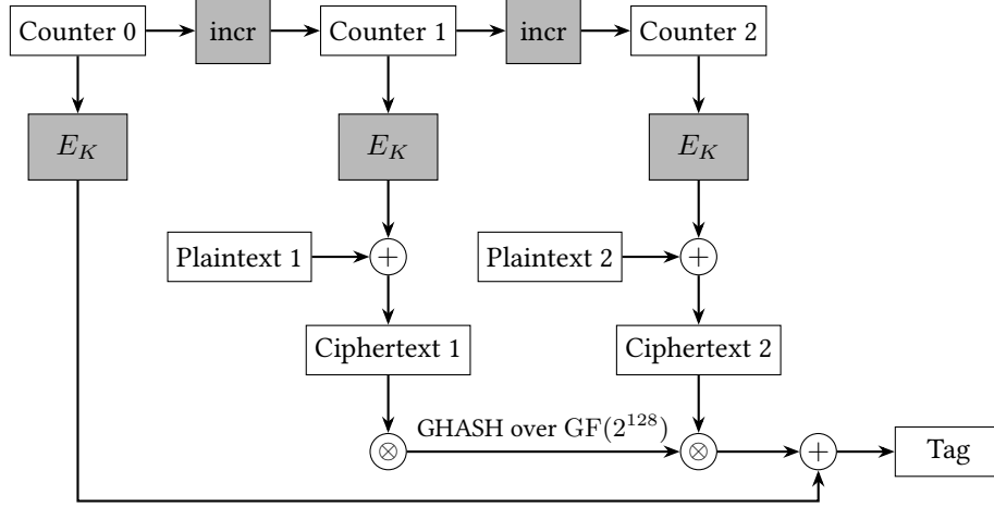
(b) AES-128-GCM: the block cipher E_K runs in counter mode to produce a keystream, and a separate GHASH multiplication in GF(2^{128}) authenticates the ciphertext into the tag.
