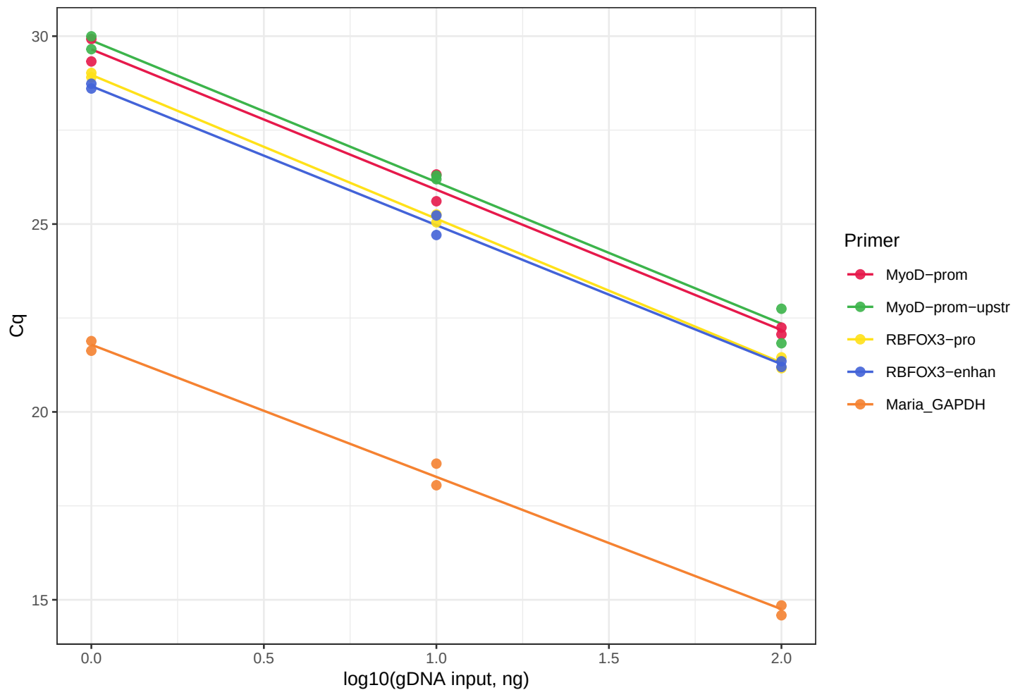
Negative-control primer standard curves (Maria gDNA, PowerUp SYBR)
