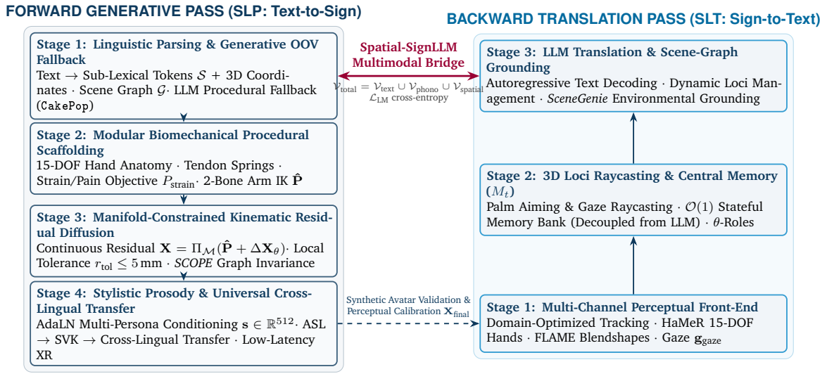
Figure 1: The Unified Bidirectional Spatial Foundation Pipeline with the Spatial-SignLLM Multimodal Bridge.
