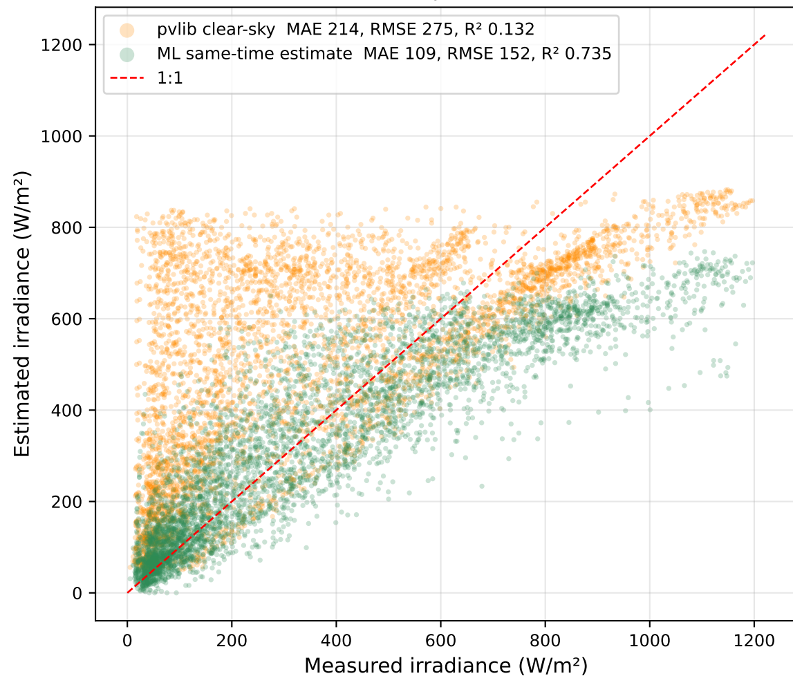
Clean-sensor months (Jan, Feb, Nov, Dec 2023)
