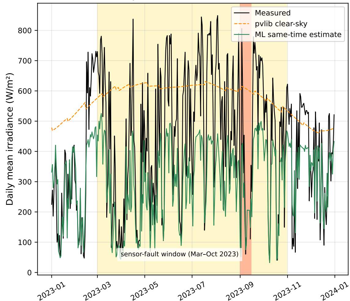
Daily mean irradiance across 2023
