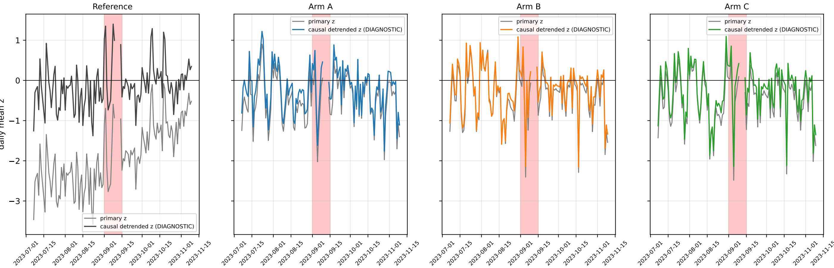
Primary vs causal-detrended residual z around the Saola PROXY EVENT WINDOW (red) — detrended series is DIAGNOSTIC ONLY, not a detector and not an Objective 2 result
