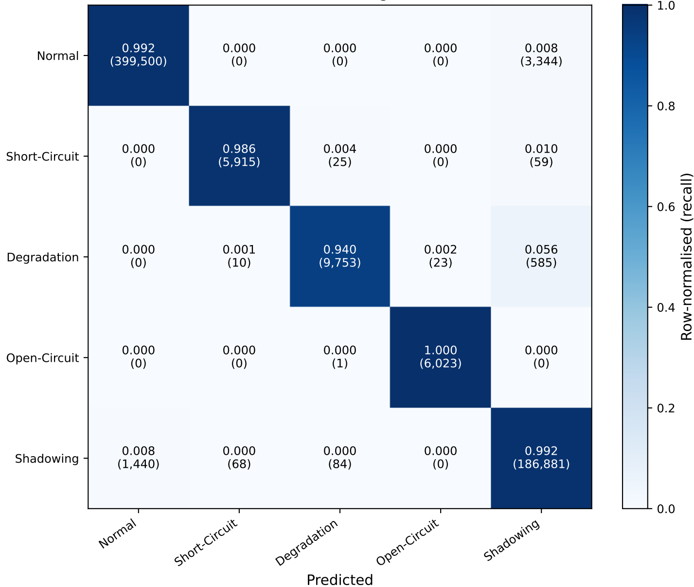
Pooled out-of-fold confusion matrix — best configuration (Electrical + irradiance, MLP)
