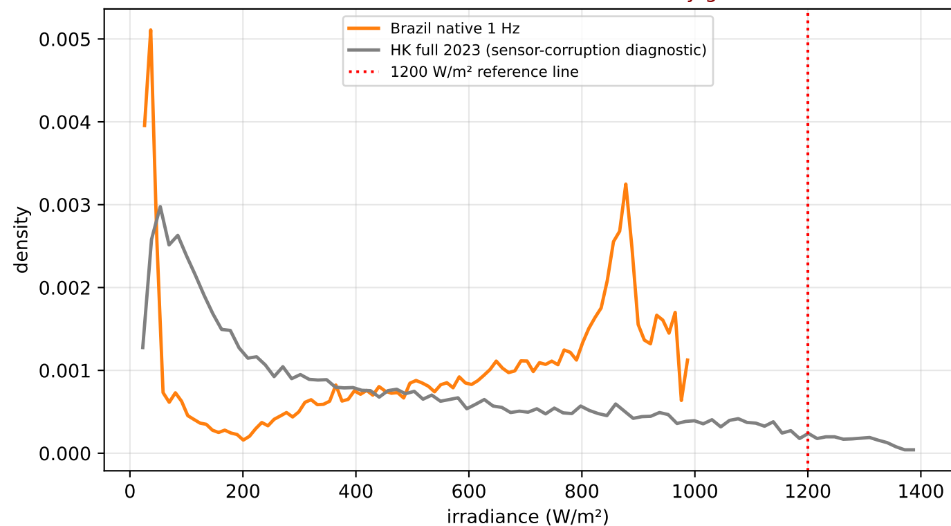
Irradiance — full 2023, KNOWN SENSOR CORRUPTION EXCLUDED from the transfer-feasibility gate
