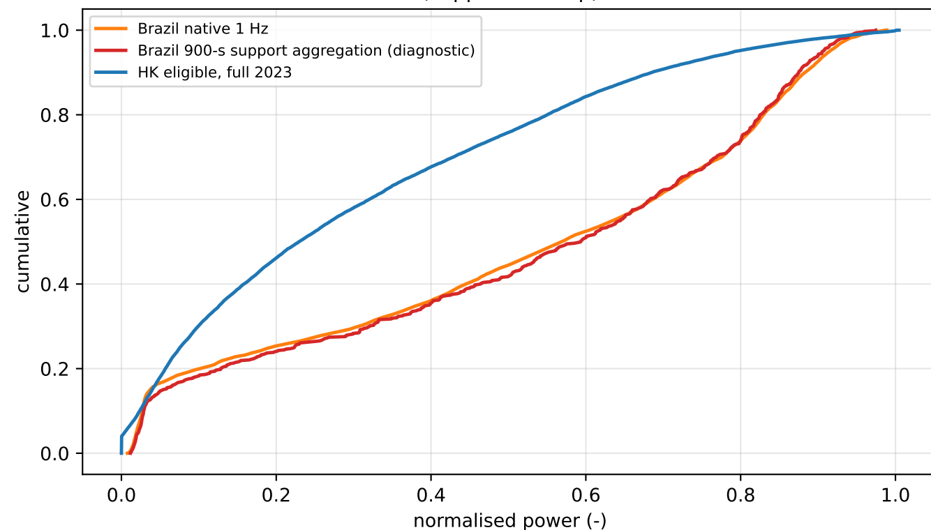
Normalised power — empirical CDF (support overlap)
