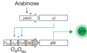
c Activator-only system
