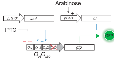
d Repressor-activator system
