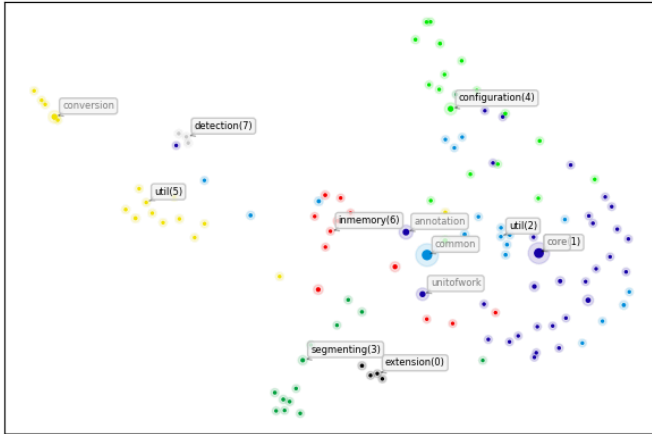
Java Packages dependency graph node embeddings Silhouette Score (aim higher)=0.2006, Davies-Bouldin Score (aim lower)=1.8807 node2vec -> UMAP
