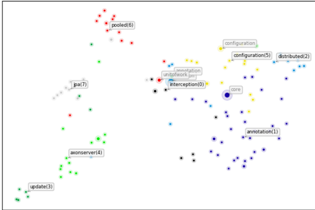
Java Packages dependency graph node embeddings Silhouette Score (aim higher)=0.2038, Davies-Bouldin Score (aim lower)=1.9835 node2vec -> UMAP
