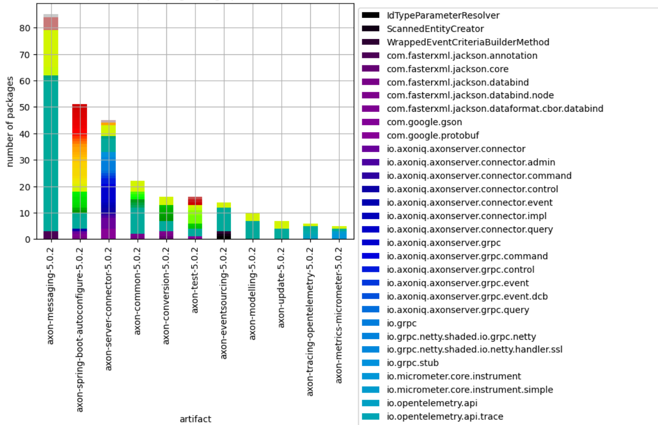
External package usage per artifact
