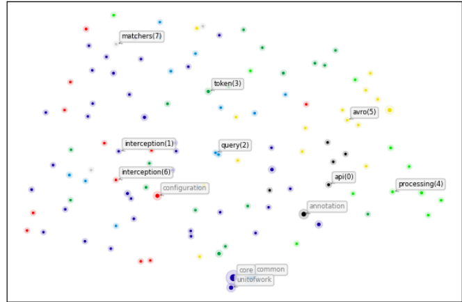
Java Packages dependency graph node embeddings Silhouette Score (aim higher)=-0.4103, Davies-Bouldin Score (aim lower)=0.0000 GraphSAGE -> UMAP
