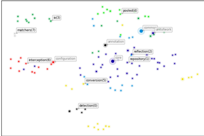
Java Packages dependency graph node embeddings Silhouette Score (aim higher)=0.2167, Davies-Bouldin Score (aim lower)=1.8588 node2vec -> UMAP
