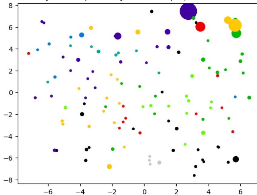
Java Package positioned by their dependency relationships (HashGNN node embeddings + t-SNE)
