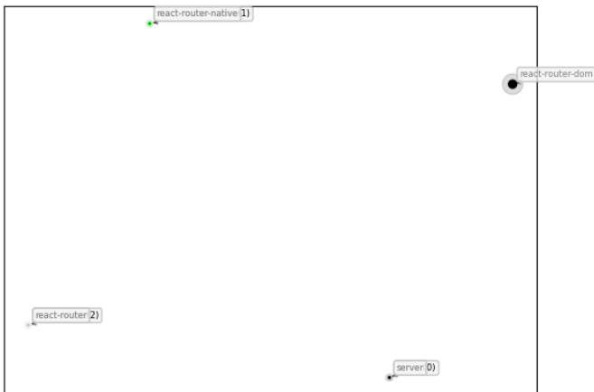
TypeScript Modules dependency graph node embeddings Silhouette Score (aim higher)=0.5000, Davies-Bouldin Score (aim lower)=0.0036 node2vec -> UMAP
