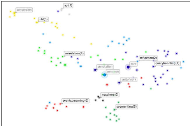
Java Packages dependency graph node embeddings Silhouette Score (aim higher)=0.2006, Davies-Bouldin Score (aim lower)=1.8875 node2vec -> UMAP
