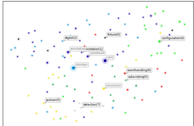
Java Packages dependency graph node embeddings Silhouette Score (aim higher)=-0.3598, Davies-Bouldin Score (aim lower)=0.0000 GraphSAGE -> UMAP
