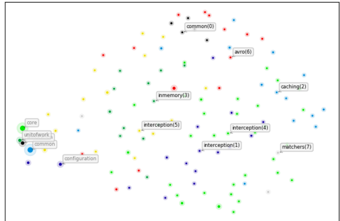
Java Packages dependency graph node embeddings Silhouette Score (aim higher)=-0.3744, Davies-Bouldin Score (aim lower)=0.0000 GraphSAGE -> UMAP
