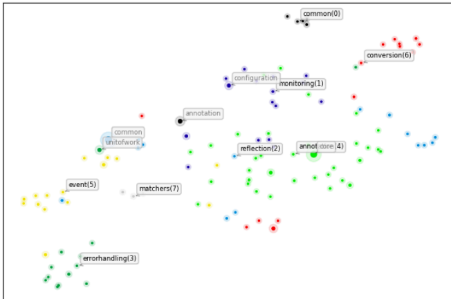
Java Packages dependency graph node embeddings Silhouette Score (aim higher)=0.2177, Davies-Bouldin Score (aim lower)=1.8572 node2vec -> UMAP
