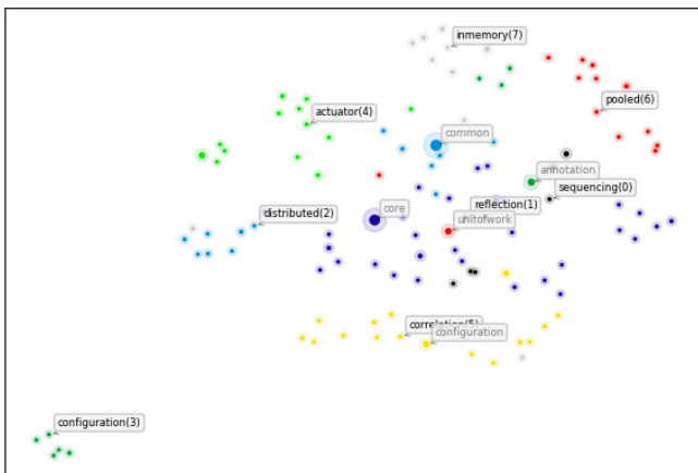
Java Packages dependency graph node embeddings Silhouette Score (aim higher)=0.1912, Davies-Bouldin Score (aim lower)=2.0185 node2vec -> UMAP
