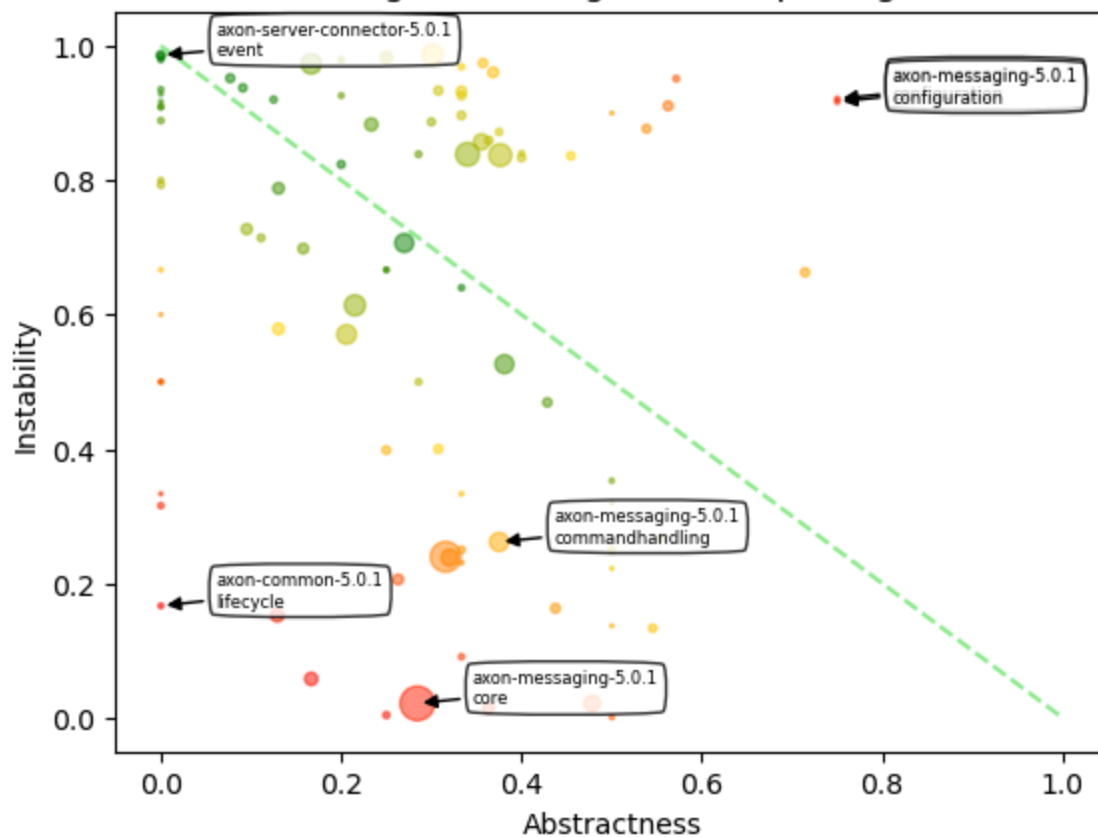
Abstractness vs. Instability ("Main Sequence") Packages including their sub-packages
