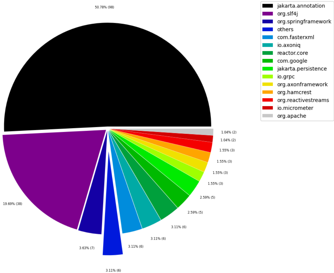
Top external package (grouped by first 2 layers) usage [%] by package (more than 0.7% overall)
