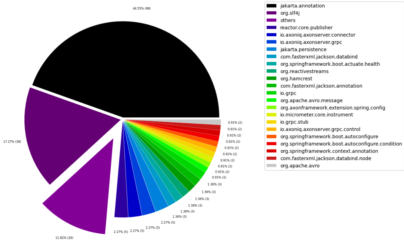
Top external package usage [%] by package (more than 0.7% overall)
