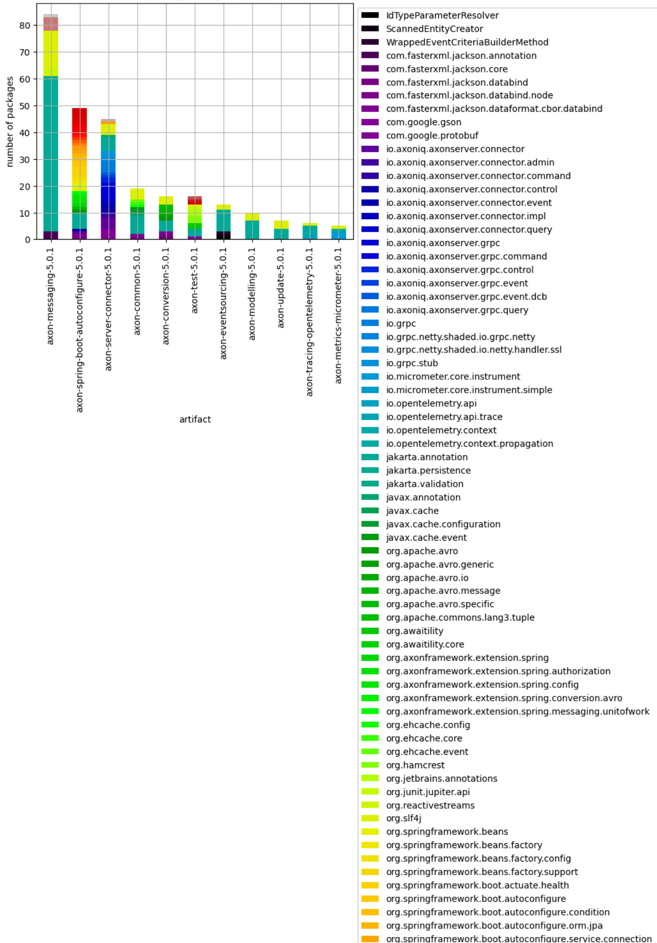
External package usage per artifact
