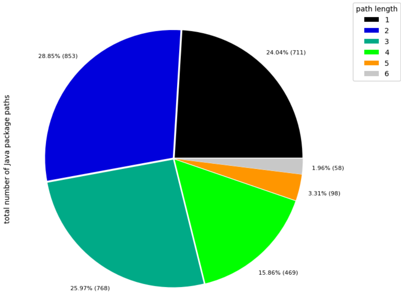
All pairs shortest path for Java package dependencies in total (pie)
