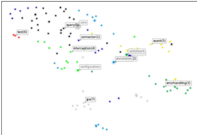
Java Packages dependency graph node embeddings Silhouette Score (aim higher)=0.1829, Davies-Bouldin Score (aim lower)=2.0163 node2vec -> UMAP
