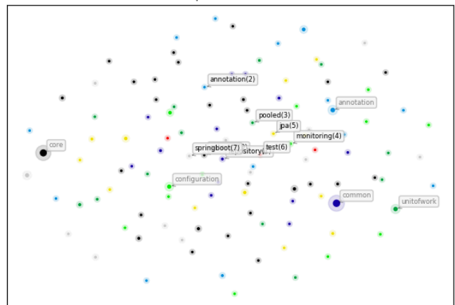
Java Packages dependency graph node embeddings Silhouette Score (aim higher)=-0.3432, Davies-Bouldin Score (aim lower)=2.0196 GraphSAGE -> UMAP
