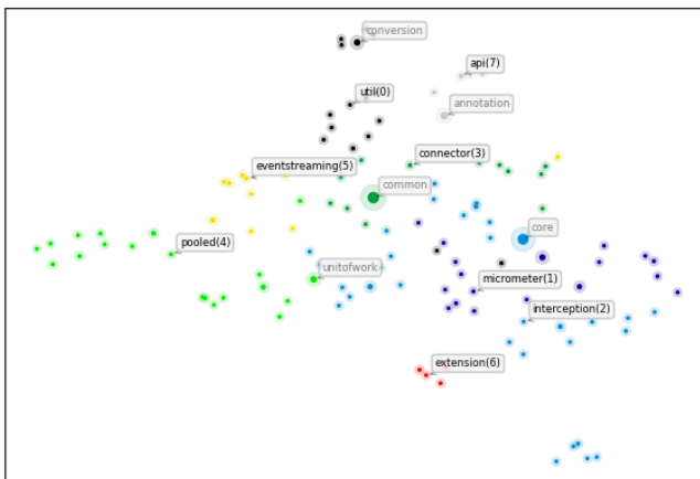
Java Packages dependency graph node embeddings Silhouette Score (aim higher)=0.2254, Davies-Bouldin Score (aim lower)=1.7625 node2vec -> UMAP
