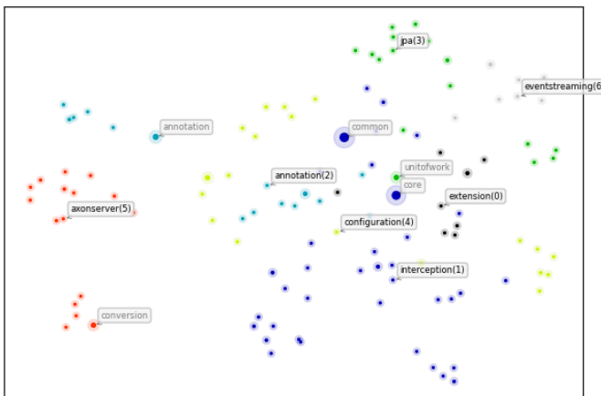
Java Packages dependency graph node embeddings Silhouette Score (aim higher)=0.1790, Davies-Bouldin Score (aim lower)=2.1055 node2vec -> UMAP
